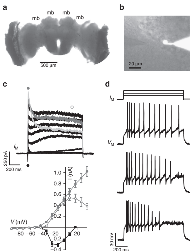
Figure 1 | Kenyon cell recordings in acutely isolated honeybee brain.
